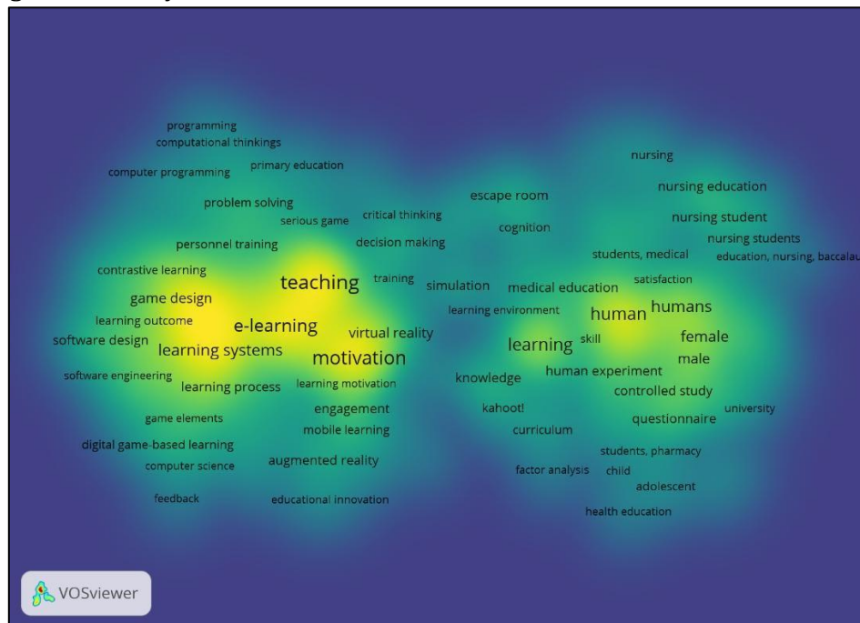
Figure 4: Density Visualization
