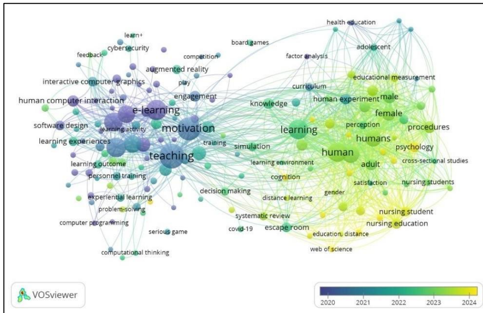
Figure 3: Overlay Visualization
