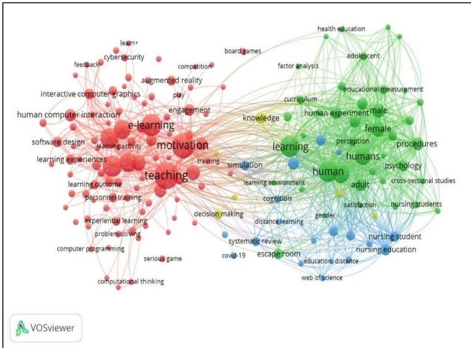
Figure 2: Network Visualization
