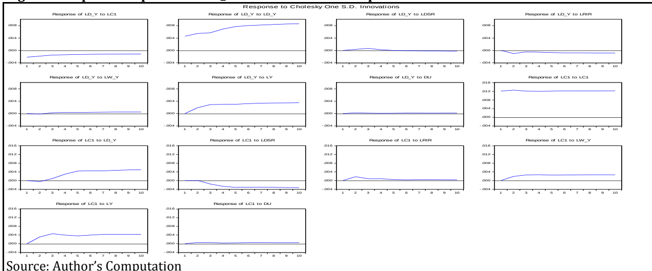
Figure 3: Impulse Responses of LD_Y and LC1 to their independent variables
